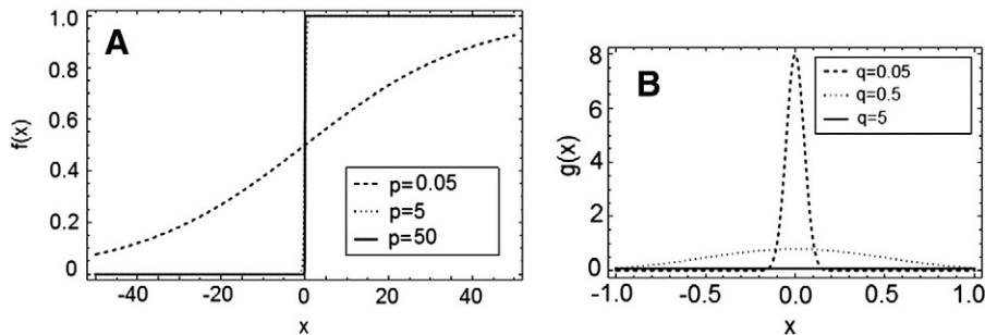
Fig. 1. (A) Three logistic functions f(t) = \frac{1}{1+e^{-pt}} as possible smoothed functions to substitute the Heaviside function H(t) and (B) three Gaussian functions g(t) = \frac{1}{q\sqrt{2\pi}} e^{-\frac{t^2}{2q^2}} as possible smoothed functions to substitute the Dirac distribution \delta(t) .
