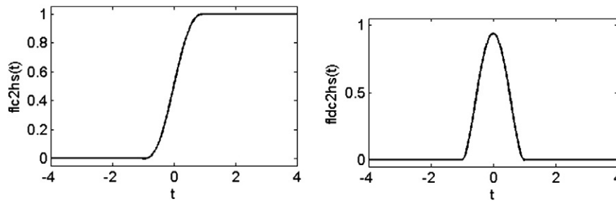
Fig. 2. Representation of f_{lc2hs}(t, p) with p = 1 (left) and f_{dc2hs}(t, q) with q = 1 (right). These smoothed functions are used by COMSOL Multiphysics as candidates to substitute Heaviside and Dirac distributions, respectively.
